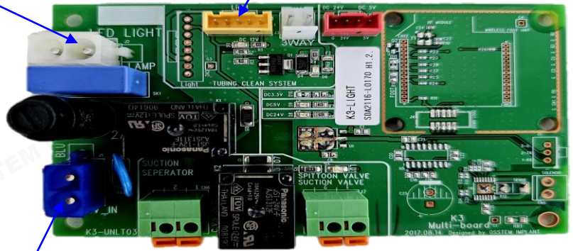
Light PCB
