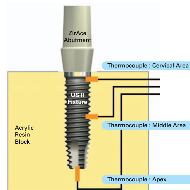
Fig 1. Schematic of locations of three temperature sensors.
